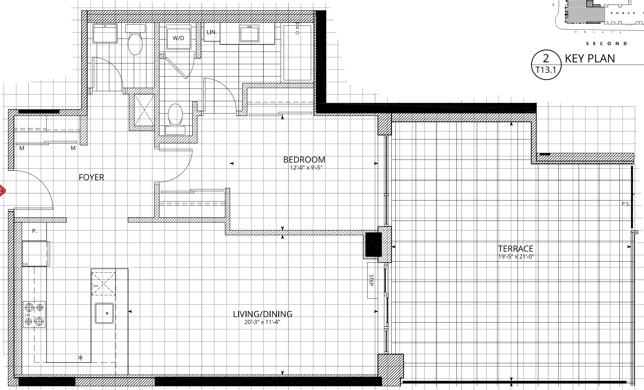
1 THE HARVEY T13.1
