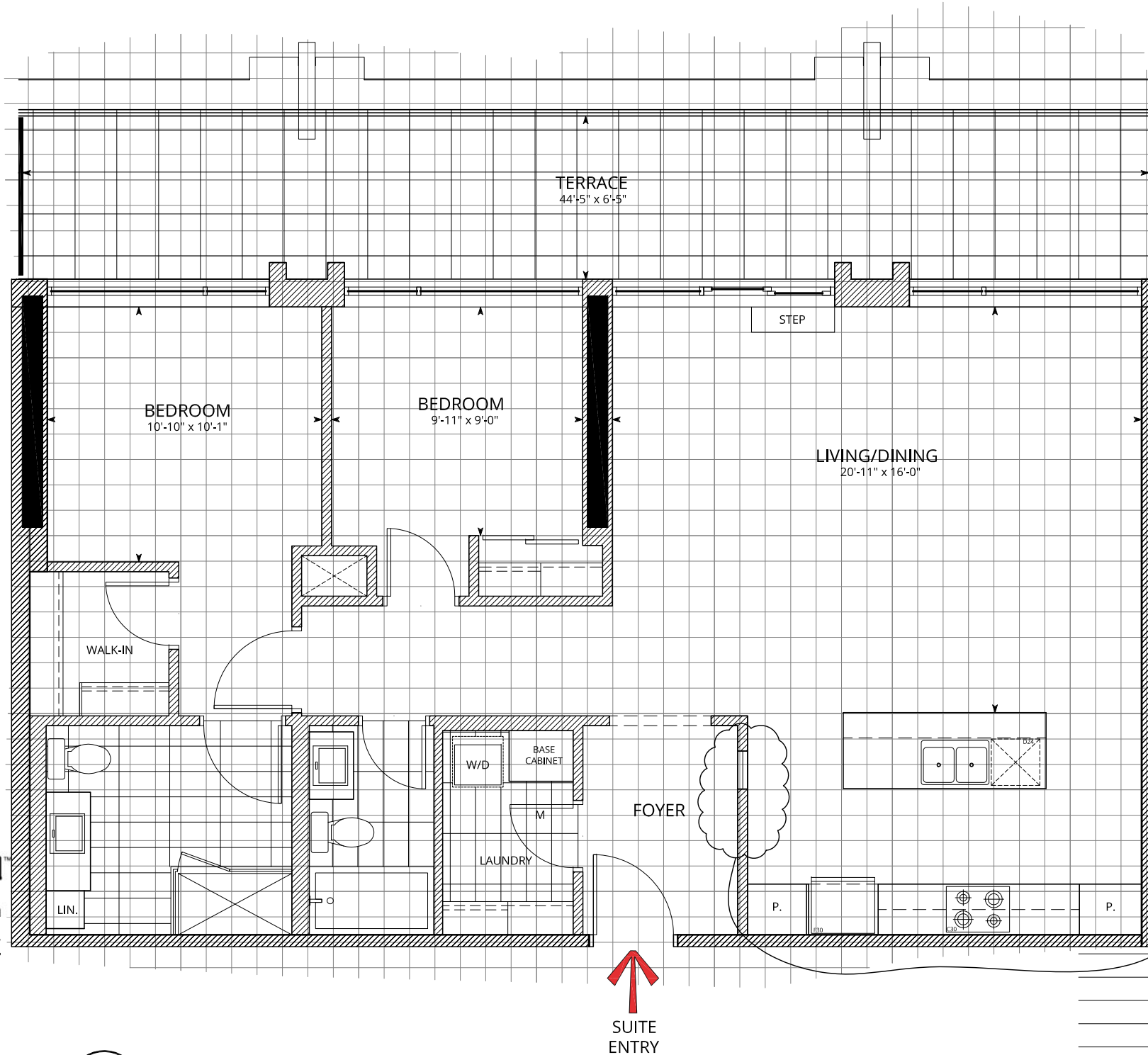
1 T1.1 THE WARRINGTON
